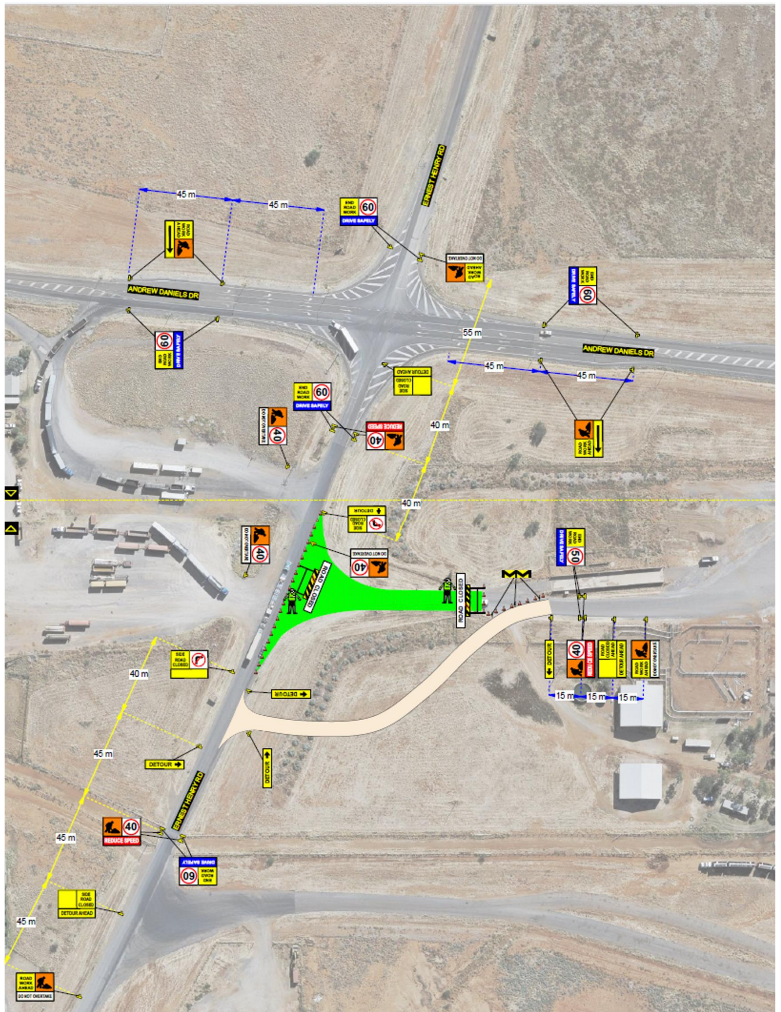
Figure 1: Salyards entrance road works and detours.
