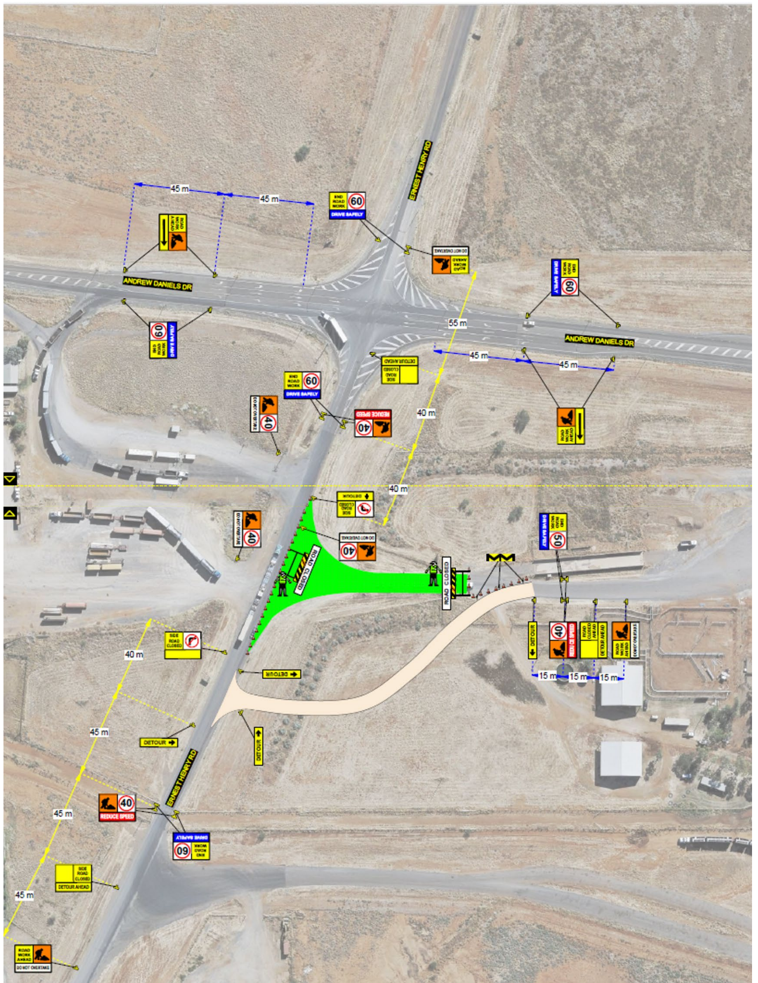
Figure 1: Saleyards entrance road works and detours.
